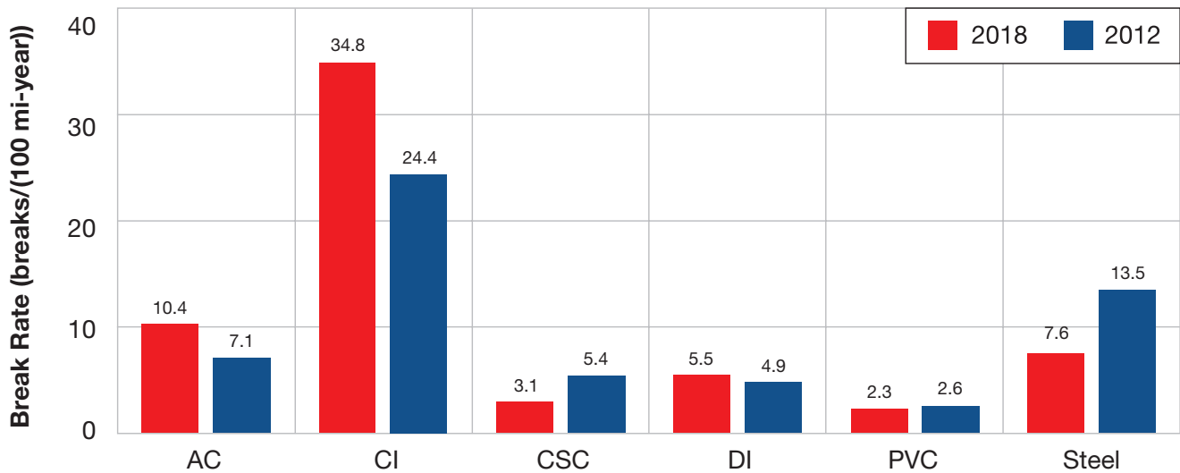
FIGURE 22: COMPARISON OF BREAK RATES OF THE 2018 AND 2012 SURVEYS
