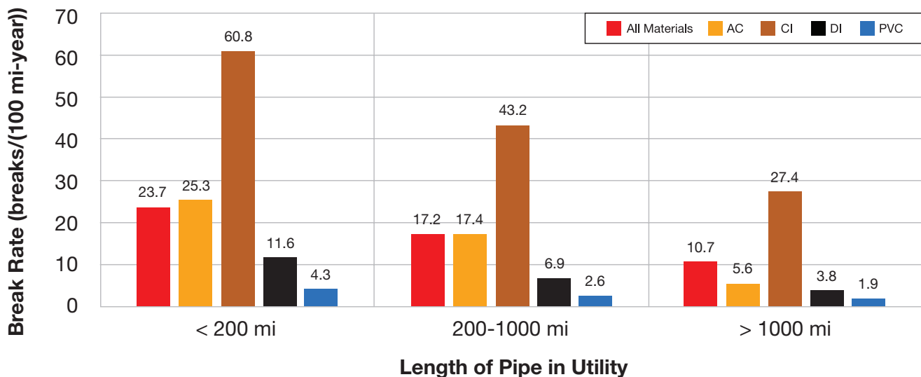
FIGURE 23: BREAK RATES BY UTILITY SIZE FROM THE BASIC SURVEY
