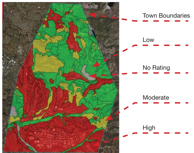
FIGURE 31: CORROSIVE SOIL RISK PLOT
