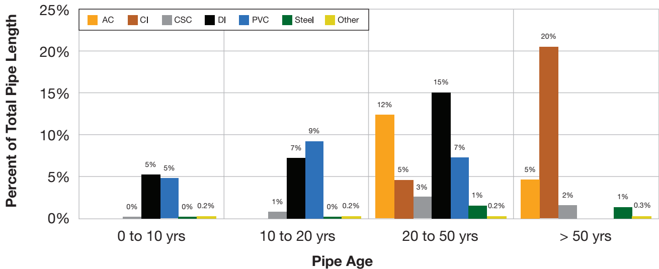
FIGURE 14: PERCENT OF TOTAL LENGTH OF PIPE BY AGE FROM THE DETAILED SURVEY
