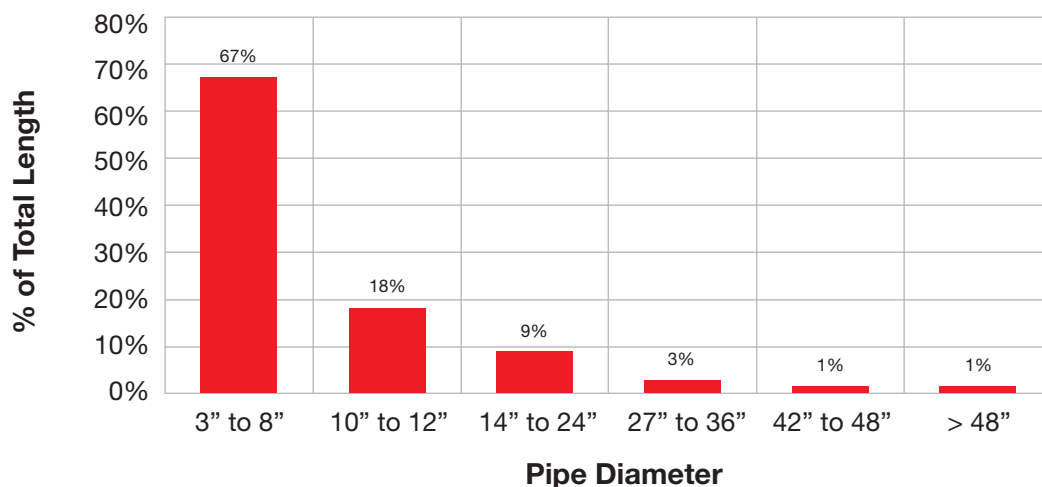
FIGURE 15: PERCENT OF TOTAL LENGTH OF PIPE BY SIZE FROM THE DETAILED SURVEY
